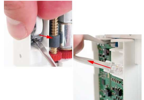
3. Unplug the RJ cable and take it out of the module. (1/2)
