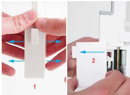
2. Slide the cover of the module off: place your thumb above the cover, pull the two sides apart and slide the cover forward
