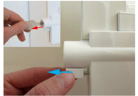
3. Take off the cap of the locking slider
