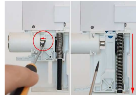
6. Push the lock a bit off the module so that the column opens
